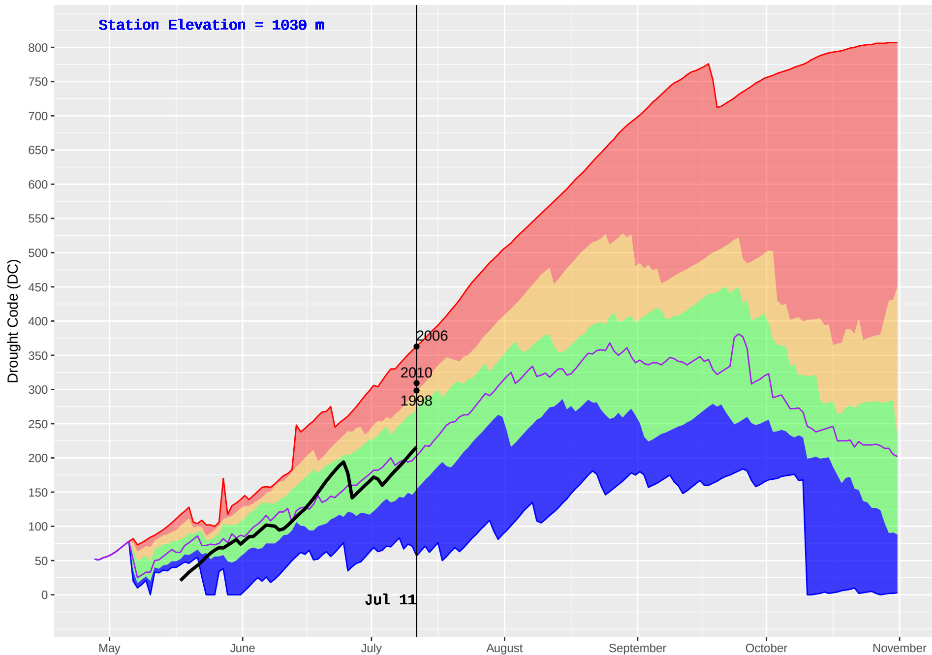
WITCH (154) : Historical (1993–2016) and Current (2018) Noon Drought Code (DC)
