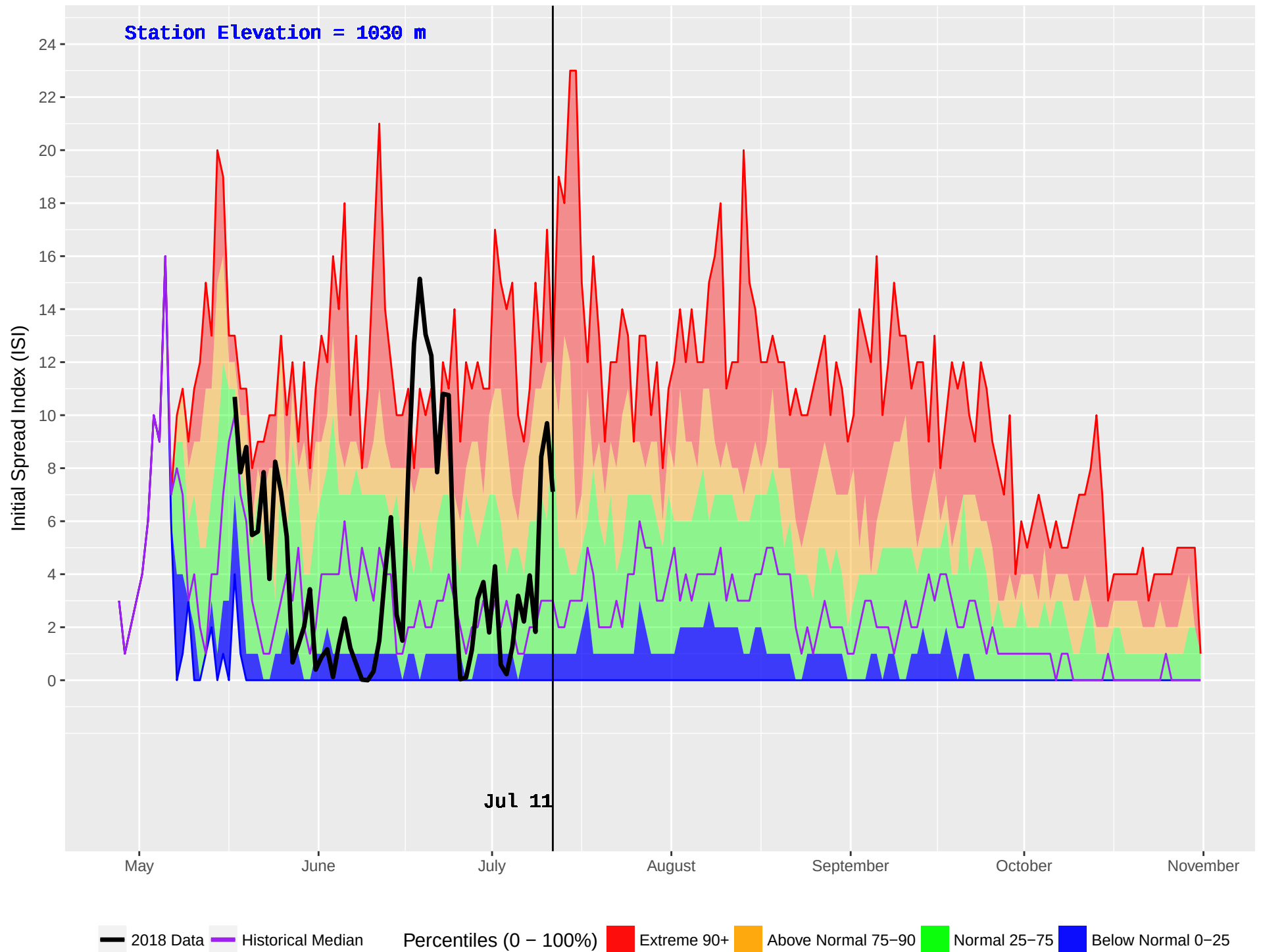
WITCH (154) : Historical (1993–2016) and Current (2018) Noon Initial Spread Index (ISI)
