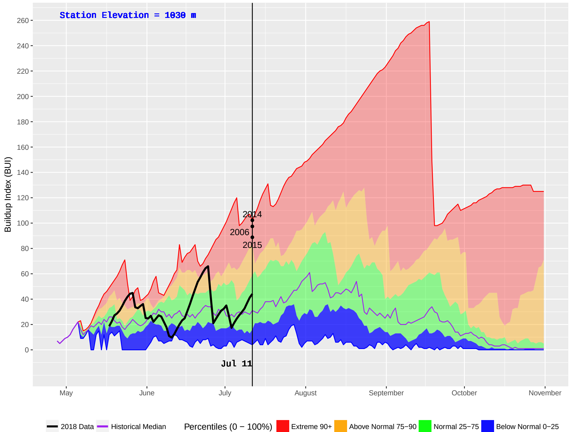
WITCH (154) : Historical (1993–2016) and Current (2018) Noon Buildup Index (BUI)
