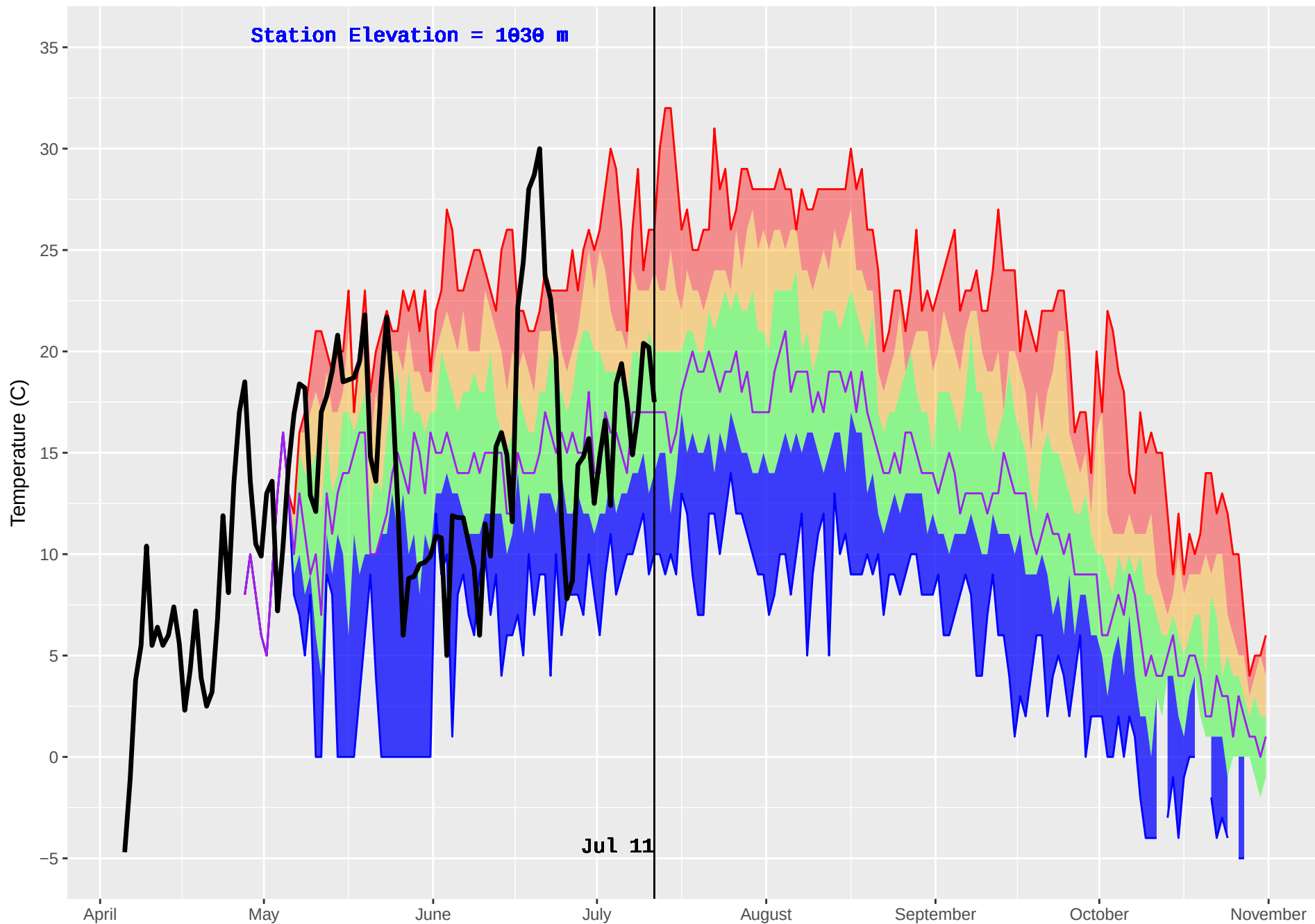
WITCH (154) : Historical (1993–2016) and Current (2018) Noon Temperature
